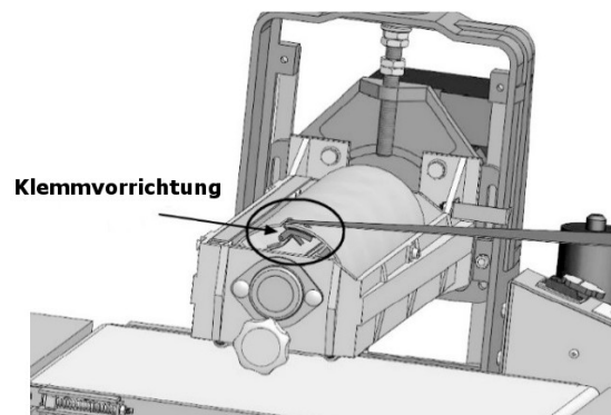
Abb. 22: Klemmvorrichtung links
